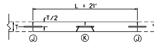
SECTION EEEE LANE REPLACEMENT L \leq 25'
